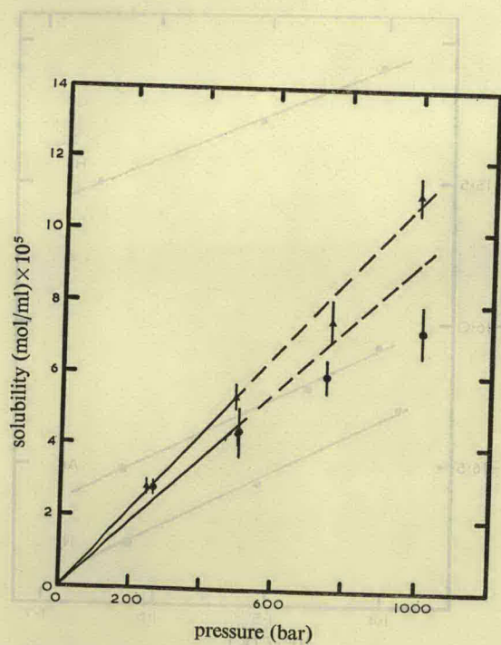
FIG. 5(b).—Solubility isotherms for the system Ar+LiNO 3 . ▲, 307°C; ●, 273°C.
